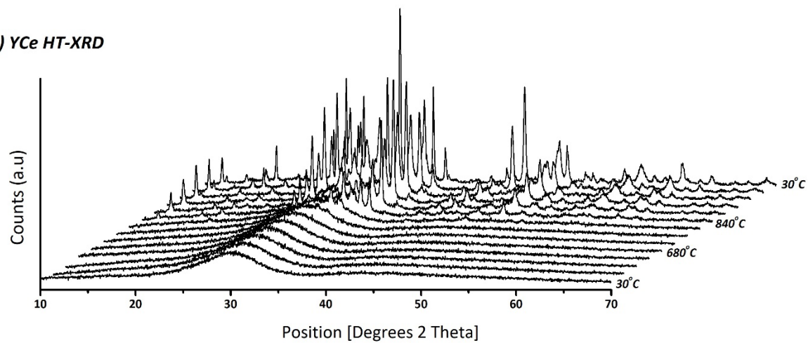
Figure 6. High Temperature X-ray Diffraction profiles of a.) HCe and b.) YCe materials from room temperature to \sim 1000^{\circ}\text{C} .
