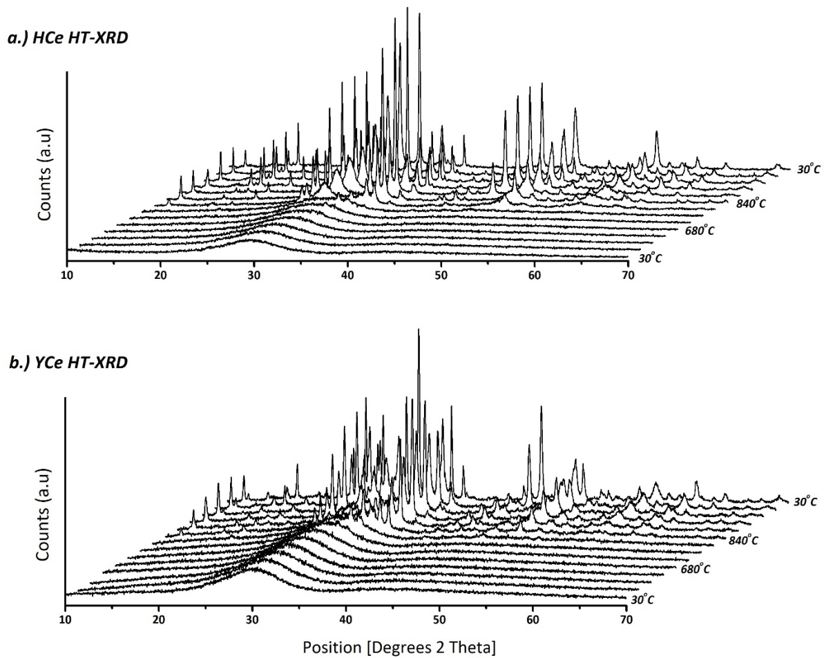
Figure 6. High Temperature X-ray Diffraction profiles of a.) HCe and b.) YCe materials from room temperature to \sim 1000^{\circ}\text{C} .
